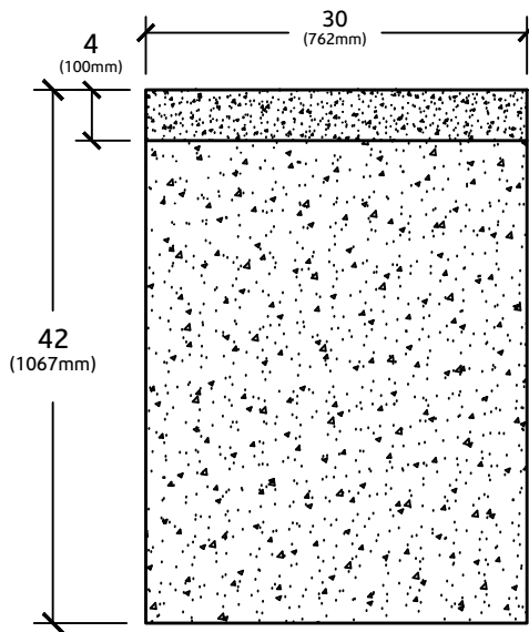
SECTION VIEW
