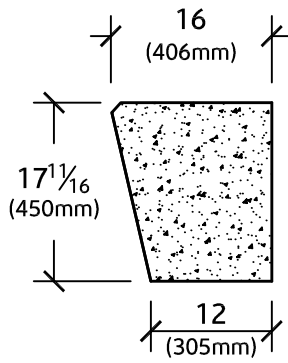
SECTION VIEW
