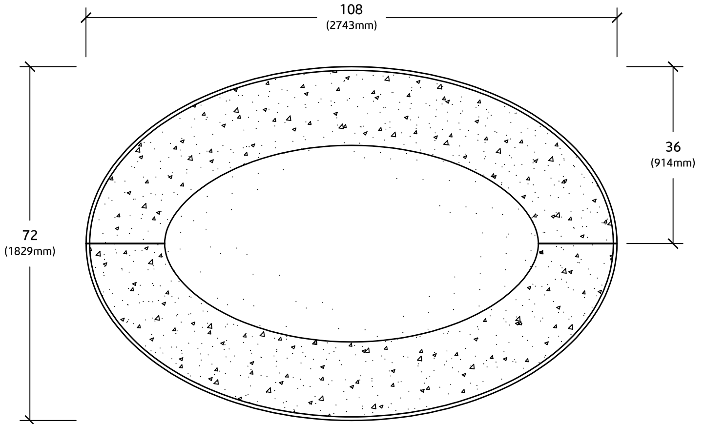
SECTION VIEW
