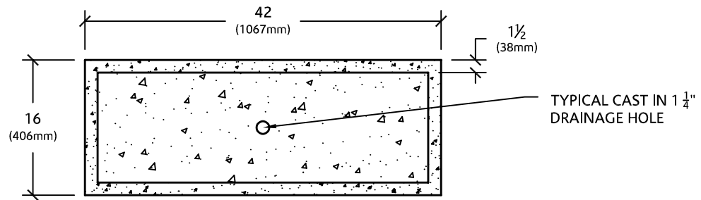
PLAN VIEW
