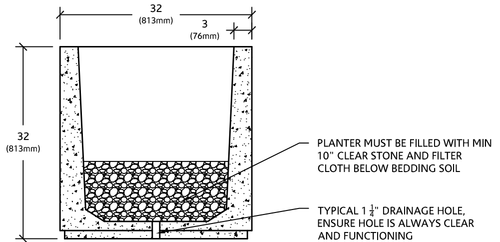
SECTION VIEW
