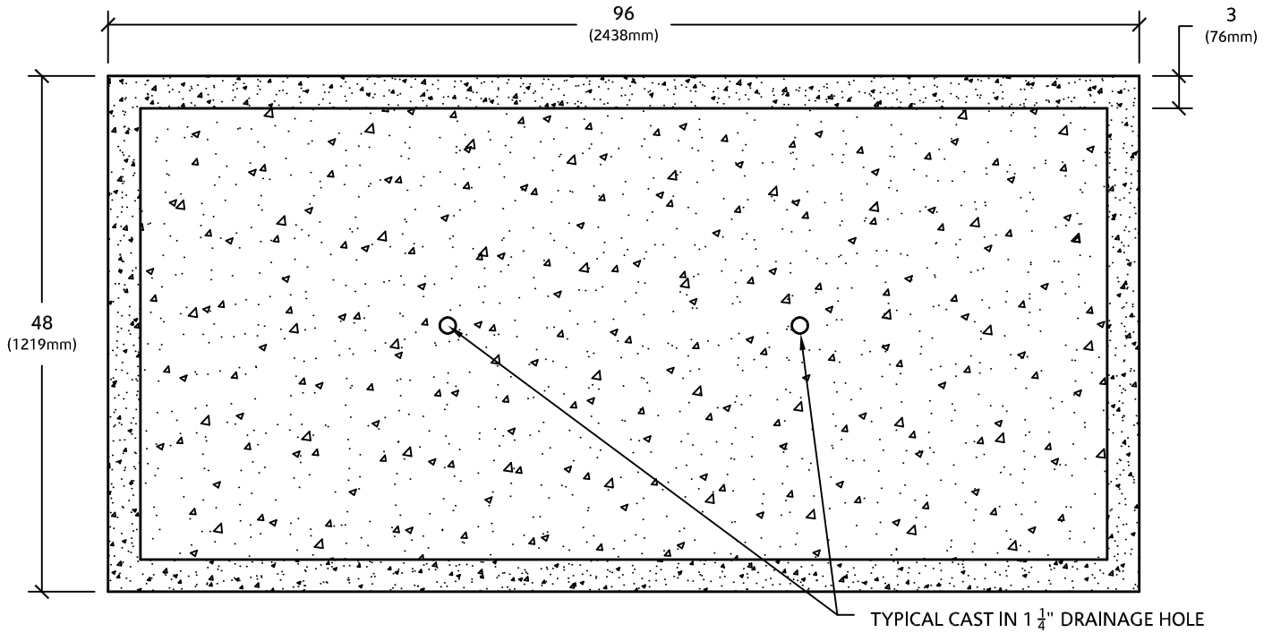
PLAN VIEW
