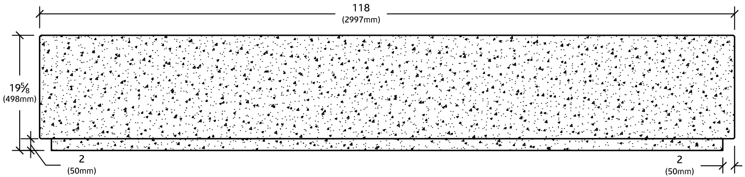
ELEVATION VIEW
