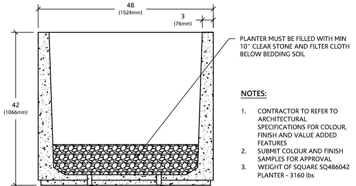
SECTION VIEW
