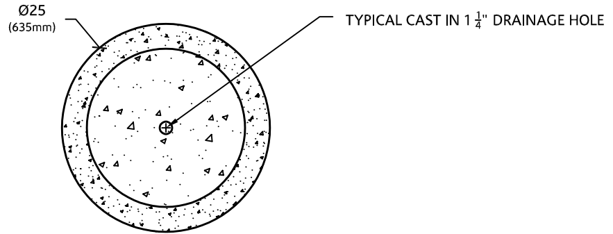
PLAN VIEW
