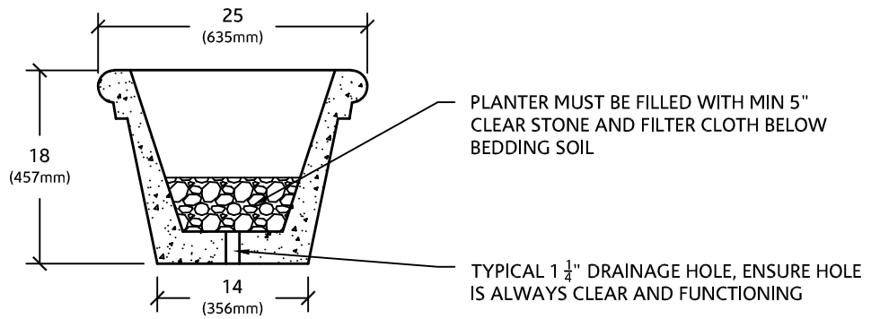
SECTION VIEW
