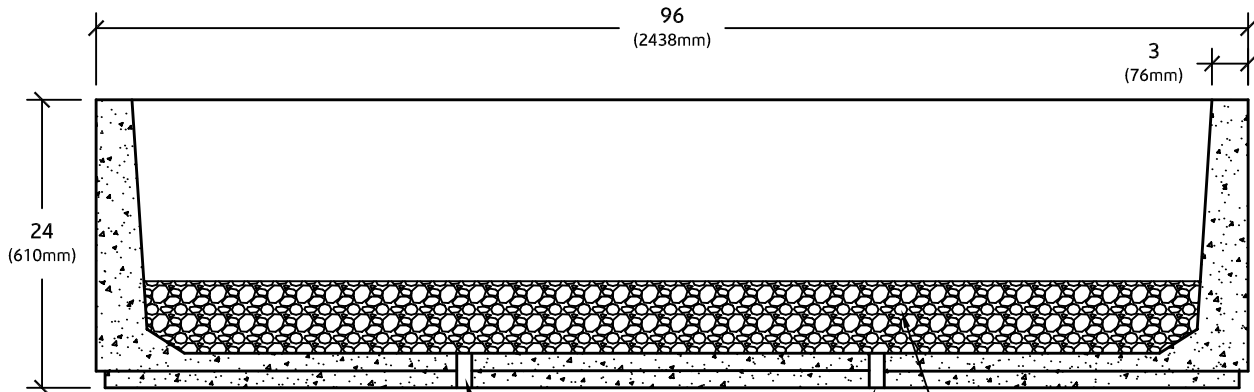
SECTION VIEW
