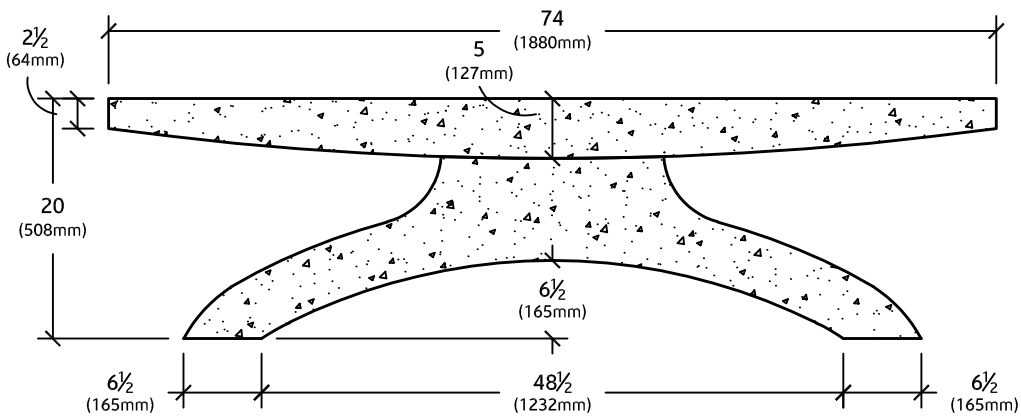
ELEVATION VIEW
