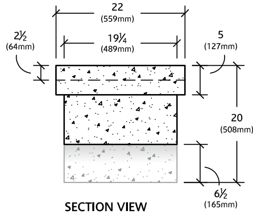
SECTION VIEW
