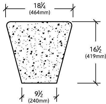
SECTION VIEW
