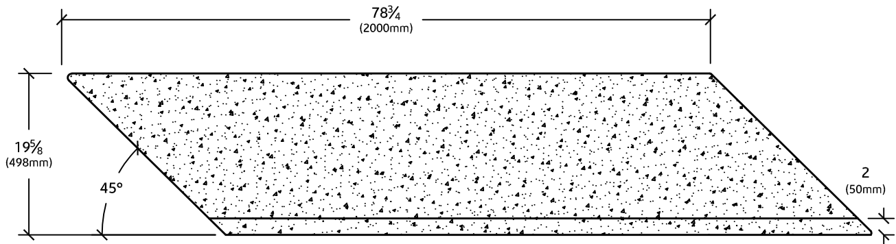
ELEVATION VIEW
