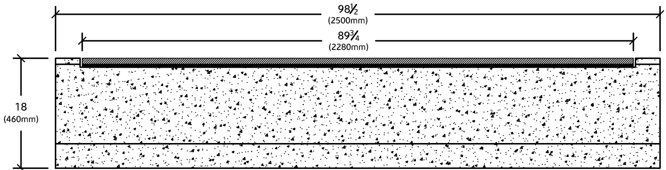
ELEVATION VIEW
