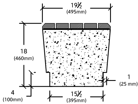
SECTION VIEW
