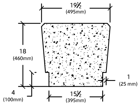
END VIEW
