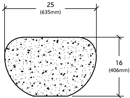
SECTION VIEW
