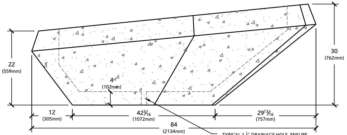
ELEVATION VIEW
