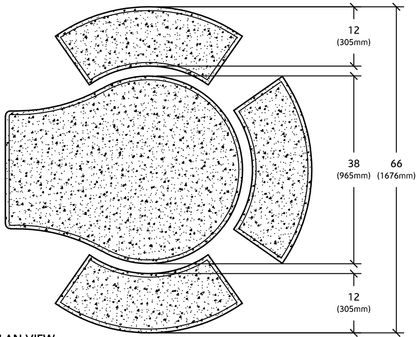
PLAN VIEW
