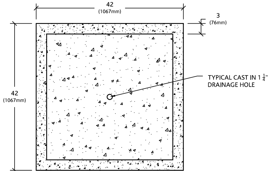
PLAN VIEW
