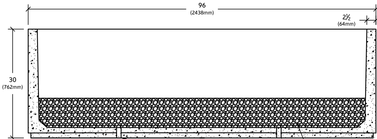
SECTION VIEW
