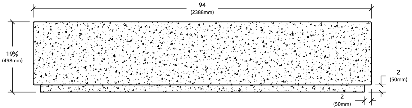
ELEVATION VIEW
