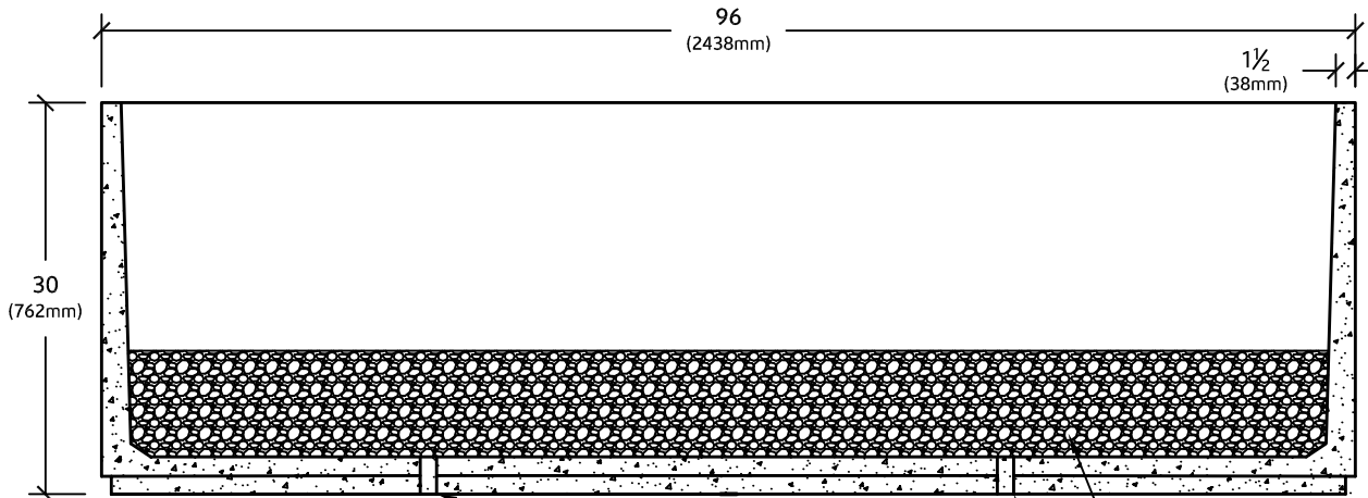
SECTION VIEW
